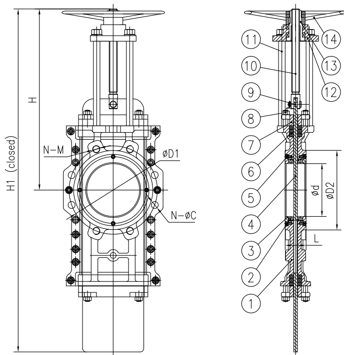
SIZE:DN50-DN150
