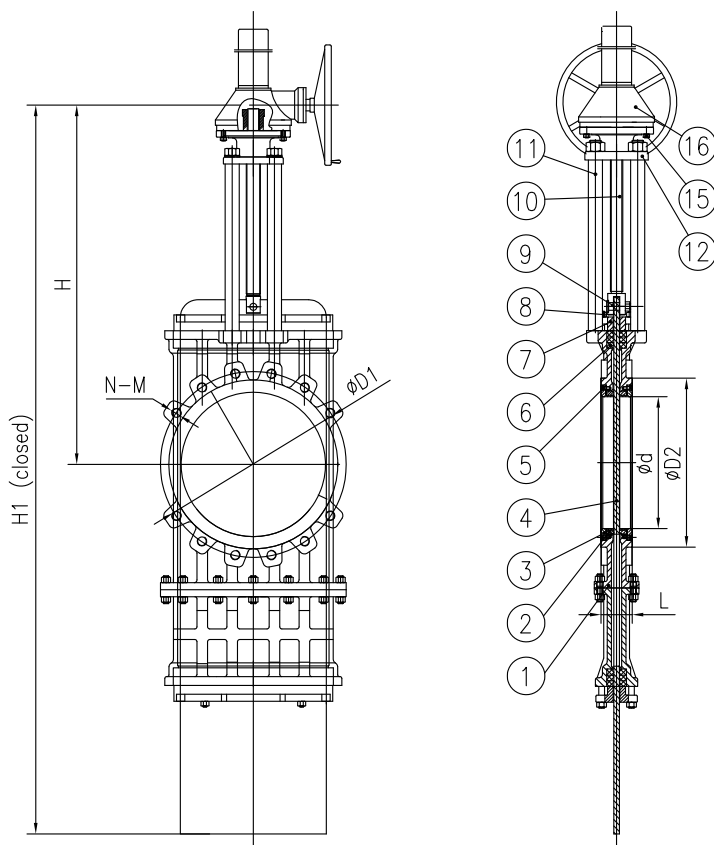
SIZE:DN200-DN600
